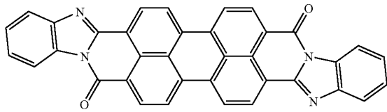
Perylene
