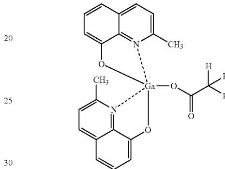
Gaq'2OAc
