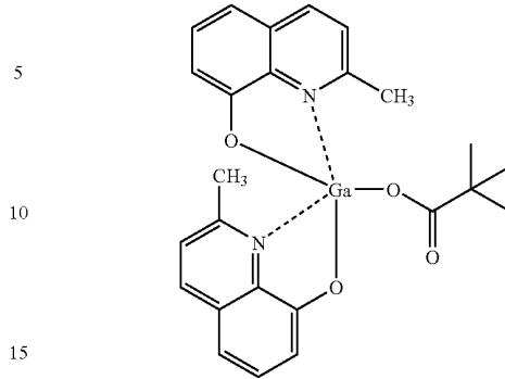
Gaq'2OPiv
